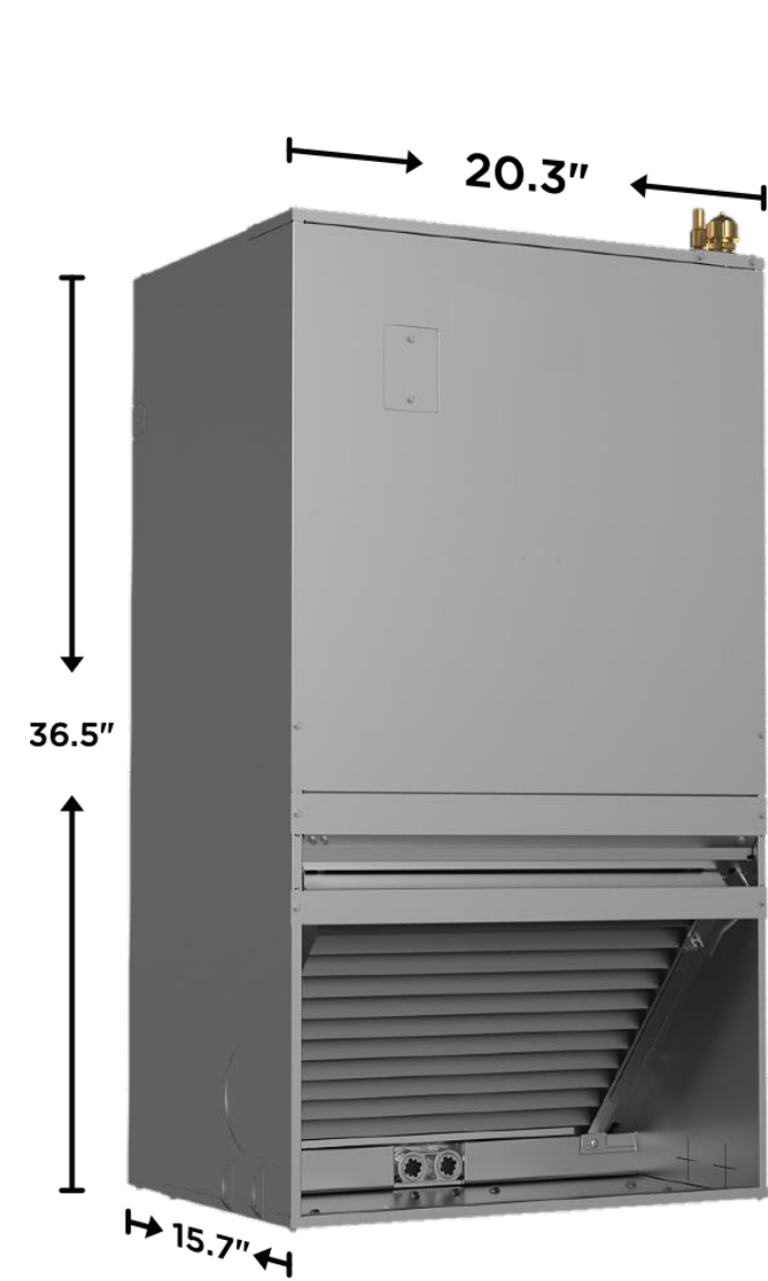
18k-24k Model
